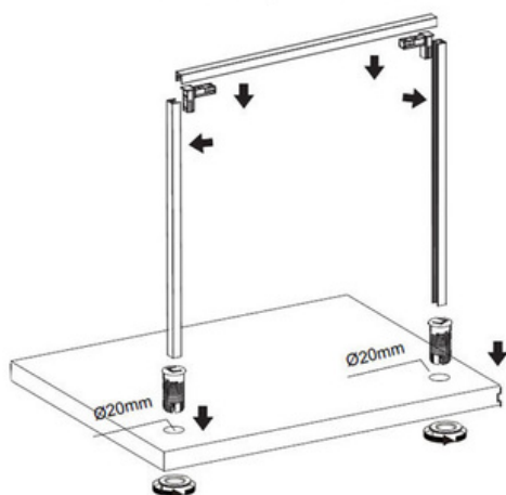
M-TRACK Gantry Installation
